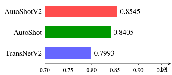
Fig. 3. F1-score comparison on SHOT. AutoShotV2 improves the reproduced AutoShot baseline by 1.40 points and the reported TransNetV2 baseline by 5.52 points.
