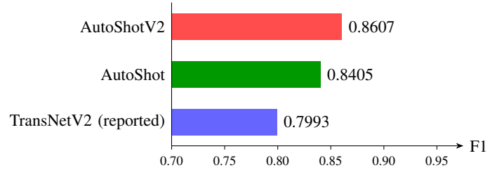
Fig. 3. F1 comparison on SHOT. AutoShotV2 outperforms the reproduced AutoShot baseline by 2.02 pp and the reported TransNetV2 baseline by 6.14 pp.
