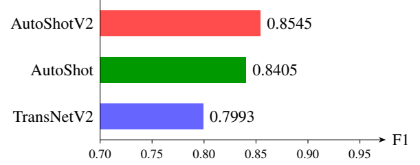
Fig. 3. F1 score comparison on SHOT. AutoShotV2 improves the reproduced AutoShot baseline by 1.40 percentage points and the reported TransNetV2 baseline by 5.52 percentage points in F1.
