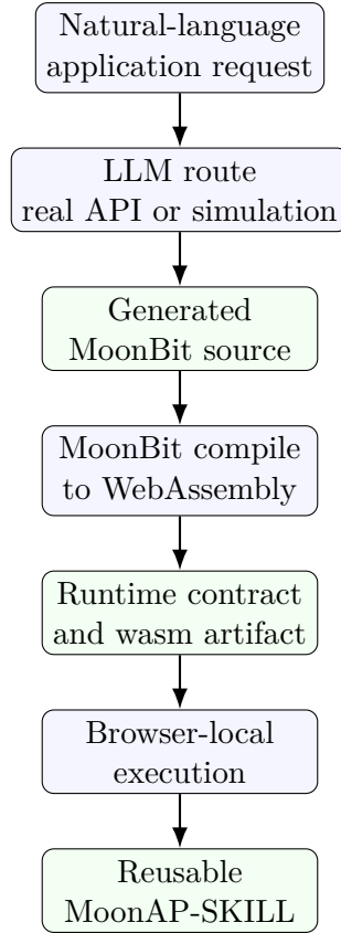
Figure 1: End-to-end MoonAP workflow. The LLM participates in source generation, while browser-local execution and artifact reuse are controlled by the host system.
