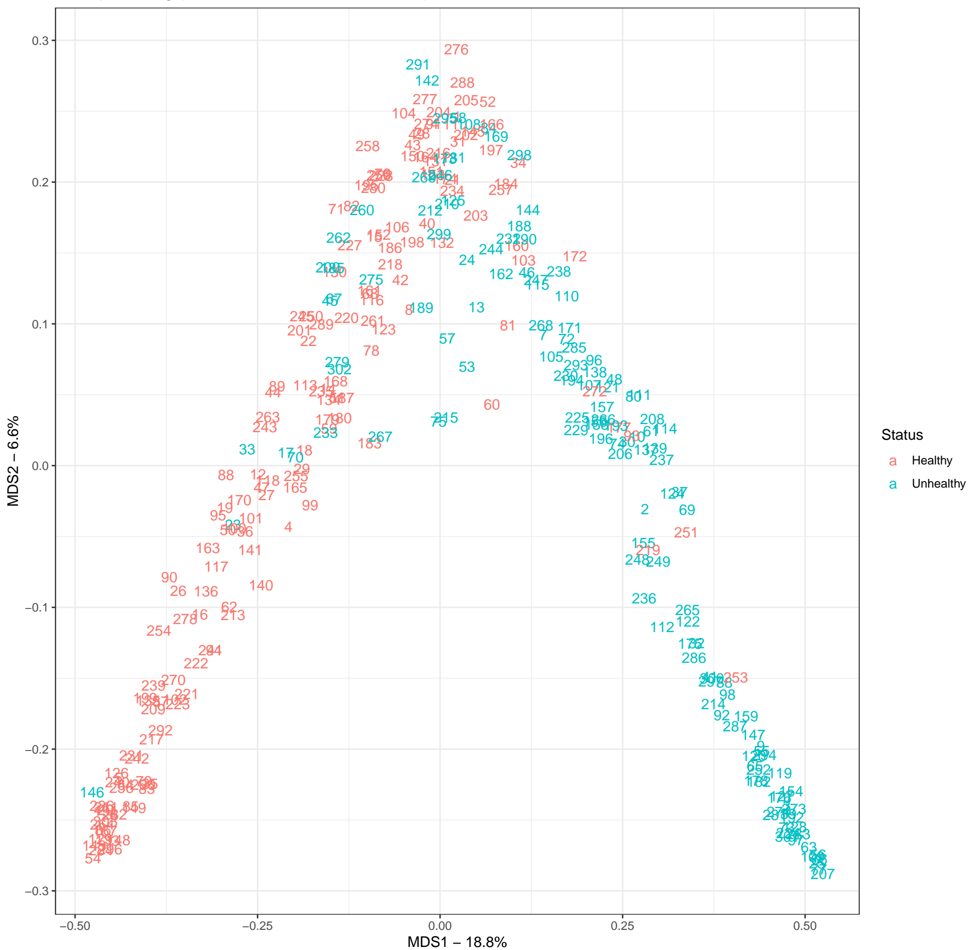
MDS plot using (1 – Random Forest Proximities)
