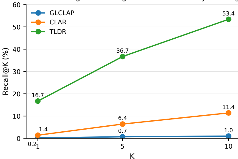
Zero-shot English ranking under Chinese-only training
