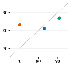
ContextASR-EN
