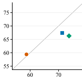
AISpeechMeeting
