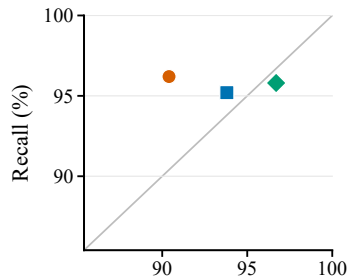
AISHELL1-NE
