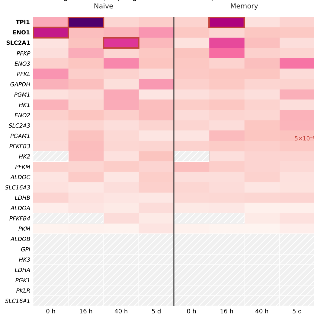
a Strongest cis-eQTL per gene and activation profile
