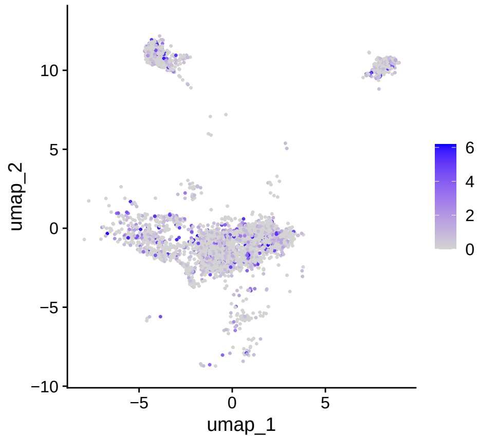
ProlifScore
