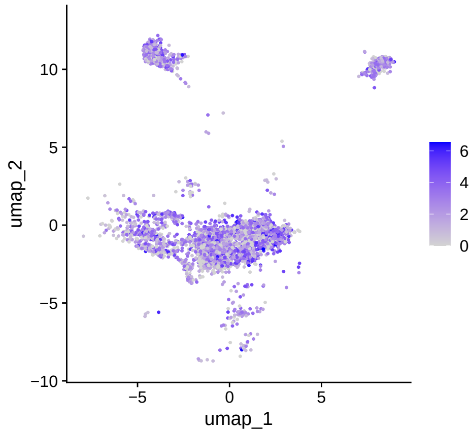
ExhaustScore
