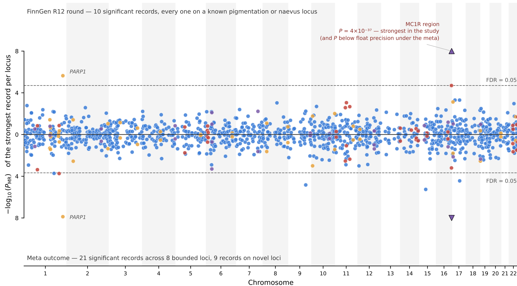
a One point per bounded locus, both outcomes
