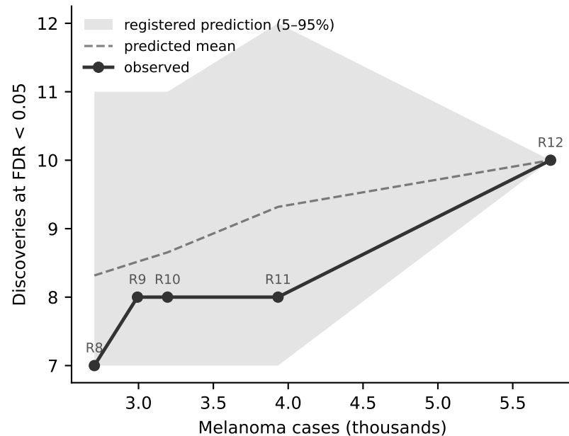
a Discoveries rise with case number
