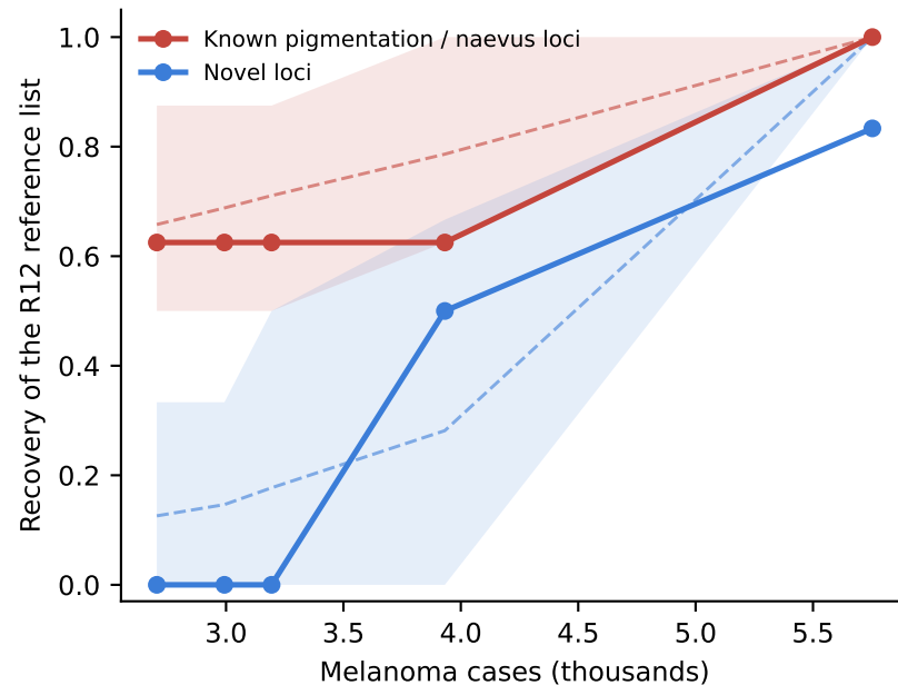
b Known loci recover early; novel loci do not (dashed = registered prediction)
