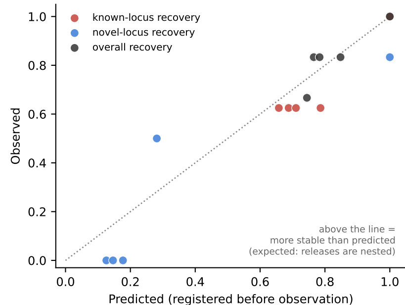
c Observed vs registered prediction
