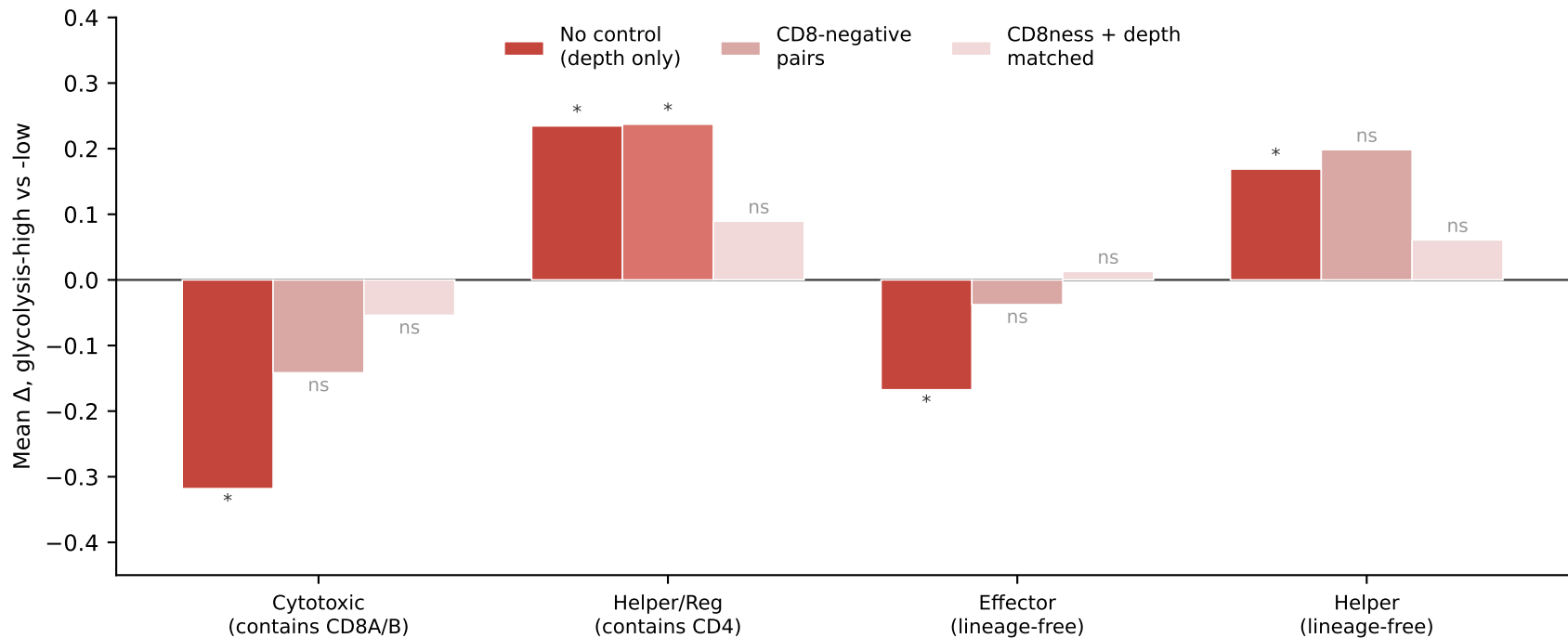
Fig S5 | A score-based split also splits lineage purity Effects collapse 75–100% once cells are matched on lineage as well as depth
