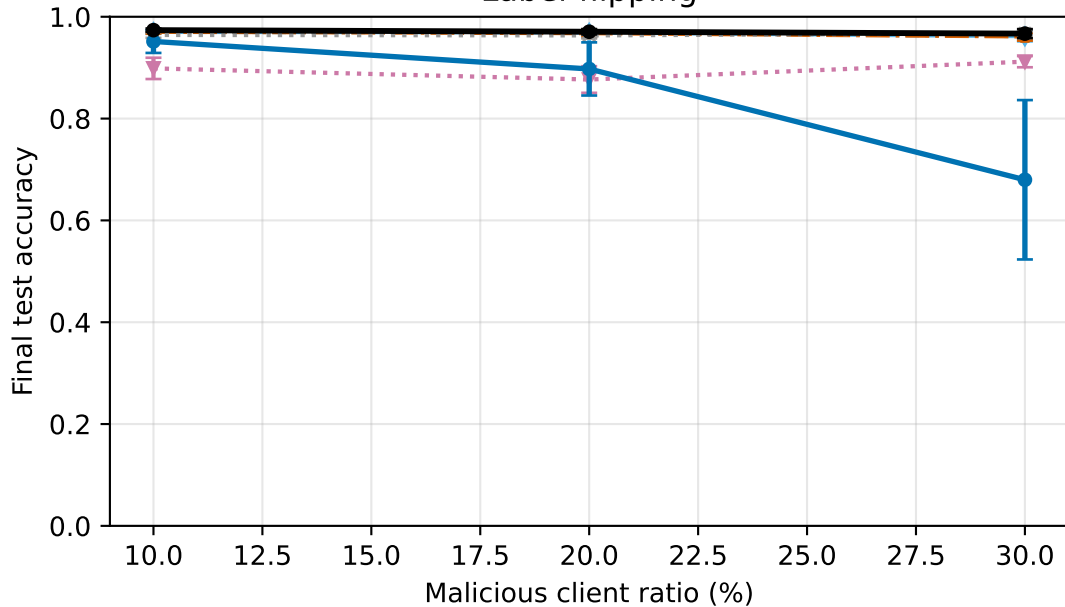
Label-flipping
