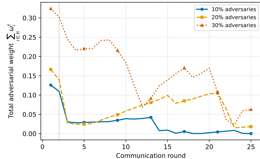
Label-flipping
