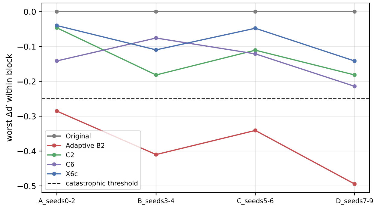
(b) worst-case \Delta d' by seed block
