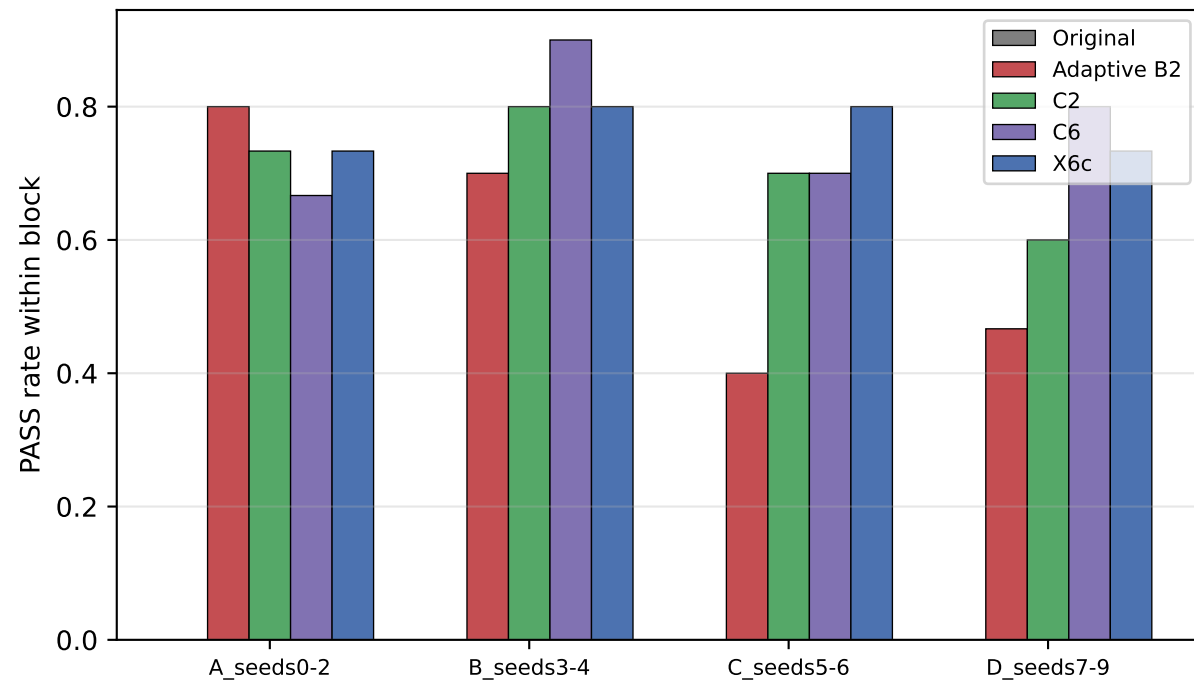
(a) PASS rate by seed block (D = unseen seeds 7-9)
