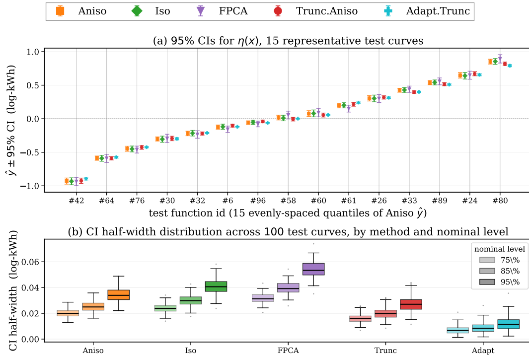
Fig 6: Pointwise CIs for \eta(x) = \langle x, \beta_0 \rangle from five methods trained on n = 2640 LCL Std households ( p = 336 time points, Haar basis with K = 32 and r = 1.5 , C_{\text{Lepski}} = 0.005 ). Trunc.Aniso and Adapt.Trunc share the default truncation level J = \lfloor n^{0.3} \rfloor . Test inputs are 100 Gaussian-process draws from \mathcal{N}(0, \hat{\Sigma}_{\text{train}}) . The shared method legend appears in the top strip. Panel (a): side-by-side 95% CIs for the fifteen test functions chosen at evenly-spaced quantiles of the Aniso point estimate. Panel (b): CI half-width distribution across all 100 test functions, grouped by method and by nominal level \{75\%, 85\%, 95\%\} (darker shading = higher nominal level); box hinges and whisker conventions are the matplotlib defaults.
