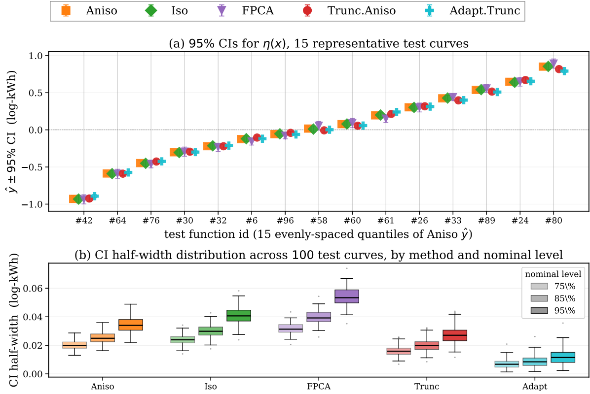
Figure 5: Pointwise CIs for \eta(x) = \langle x, \beta_0 \rangle from five methods trained on n = 2640 LCL Std households ( p = 336 time points, Haar basis with K = 32 and r = 1.5 , C_{\text{Lepski}} = 0.005 ). Trunc.Aniso and Adapt.Trunc share the default truncation level J = \lfloor n^{0.3} \rfloor . Test inputs are 100 Gaussian-process draws from \mathcal{N}(0, \hat{\Sigma}_{\text{train}}) . The shared method legend appears in the top strip. Panel (a): side-by-side 95% CIs for the fifteen test functions chosen at evenly-spaced quantiles of the Aniso point estimate. Panel (b): CI half-width distribution across all 100 test functions, grouped by method and by nominal level \{75\%, 85\%, 95\%\} (darker shading = higher nominal level); box hinges and whisker conventions are the matplotlib defaults.
