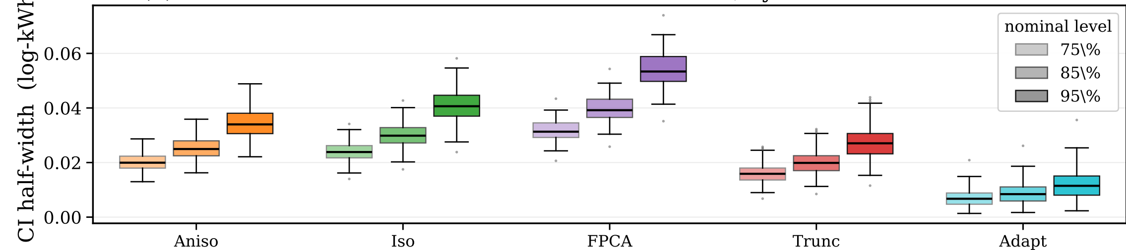
(b) CI half-width distribution across 100 test curves, by method and nominal level
