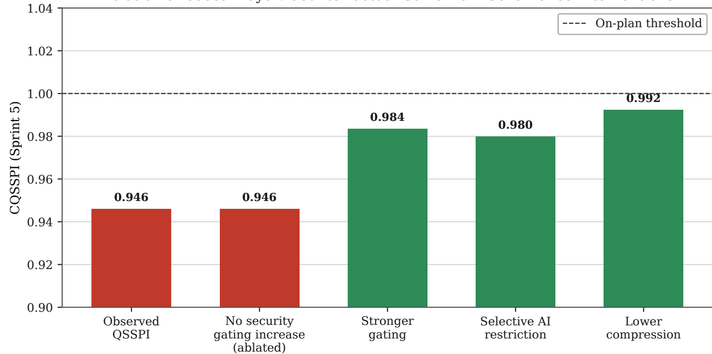
Ablation of Causal Layer: Counterfactual Gains from Governance Interventions
