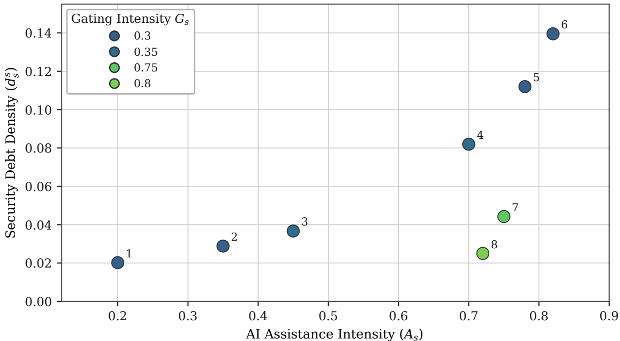
AI Assistance Intensity vs. Security Debt Density (colored by G_s )
