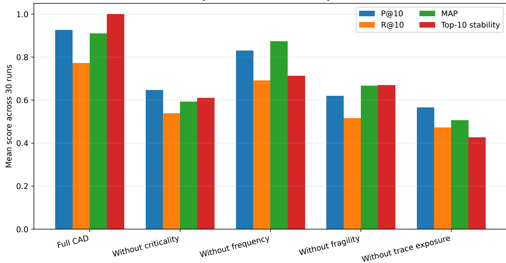
Synthetic CAD ablation analysis
