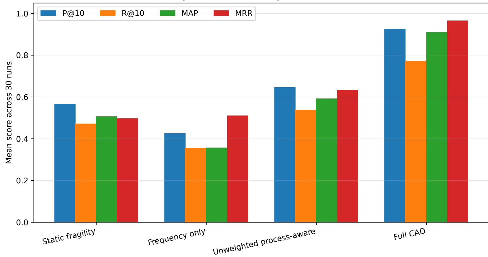
Synthetic CAD ranking effectiveness
