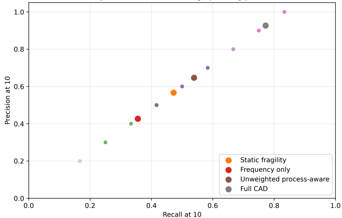
Synthetic run-level ranking operating points
