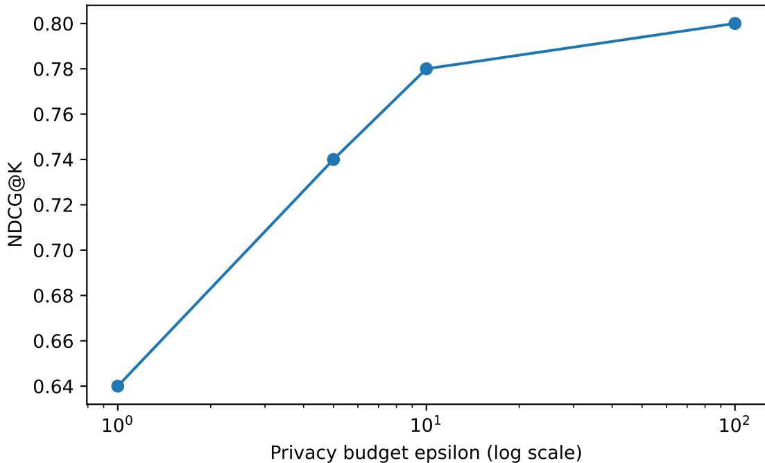
Privacy-Utility Trade-off
