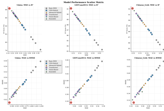
Fig. 5. Performance scatter matrix revealing model relationships across metrics with EEMD-TGNet (red circles) consistently in optimal regions
