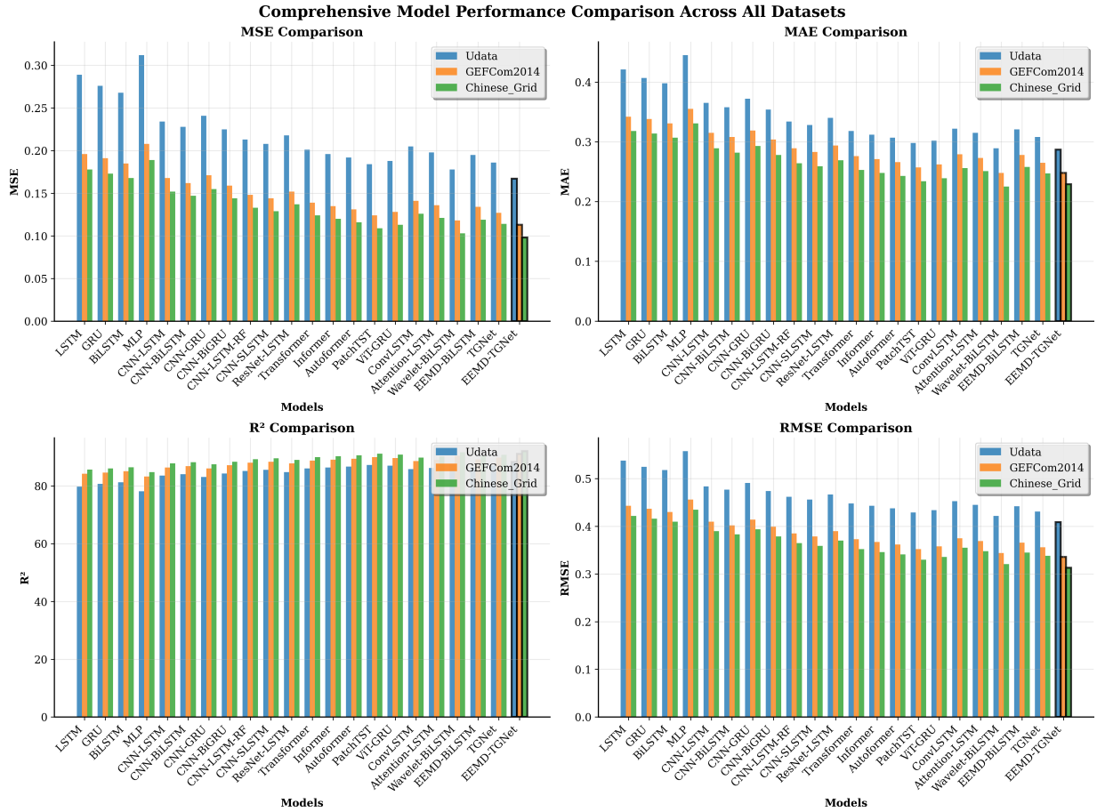
Fig. 2. Comprehensive performance comparison across 22 state-of-the-art models and all datasets. EEMD-TGNet (highlighted with black borders) consistently achieves superior performance across all metrics.
