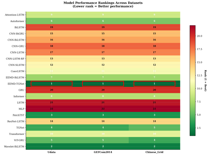
Fig. 6. Model ranking heatmap across datasets with EEMD-TGNet (red borders) achieving top rankings consistently
