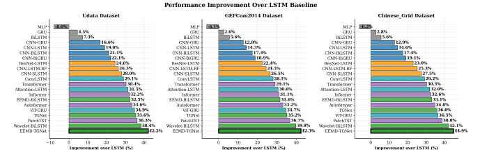
Fig. 4. Performance improvement analysis over LSTM baseline demonstrating EEMD-TGNet's superior advancement
