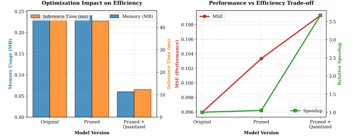
Fig. 6. Model optimization impact on efficiency and performance trade-offs
