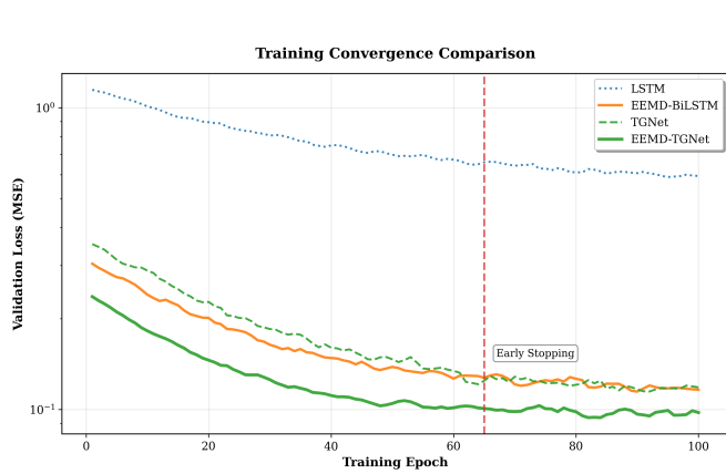
Fig. 3. Training convergence showing EEMD-TGNNet achieves faster and more stable convergence
