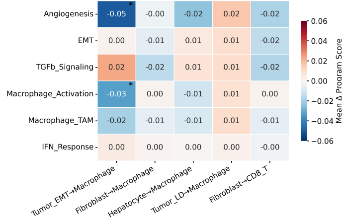
Fig. 3. Program-level mean signed counterfactual deltas (asterisk: FDR < 0.05).
