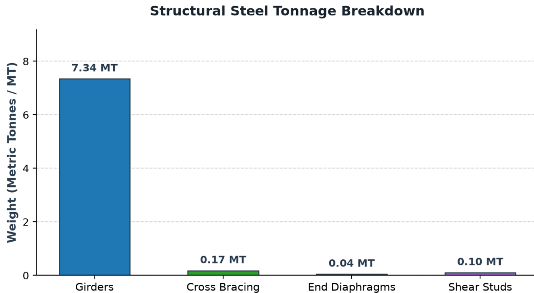
Structural Steel Tonnage Breakdown (Girders, Cross Bracing, End Diaphragms)
