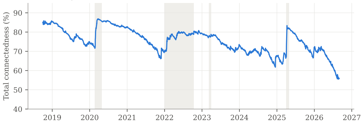
(b) Volatility connectedness, TVP-VAR (filtered)
