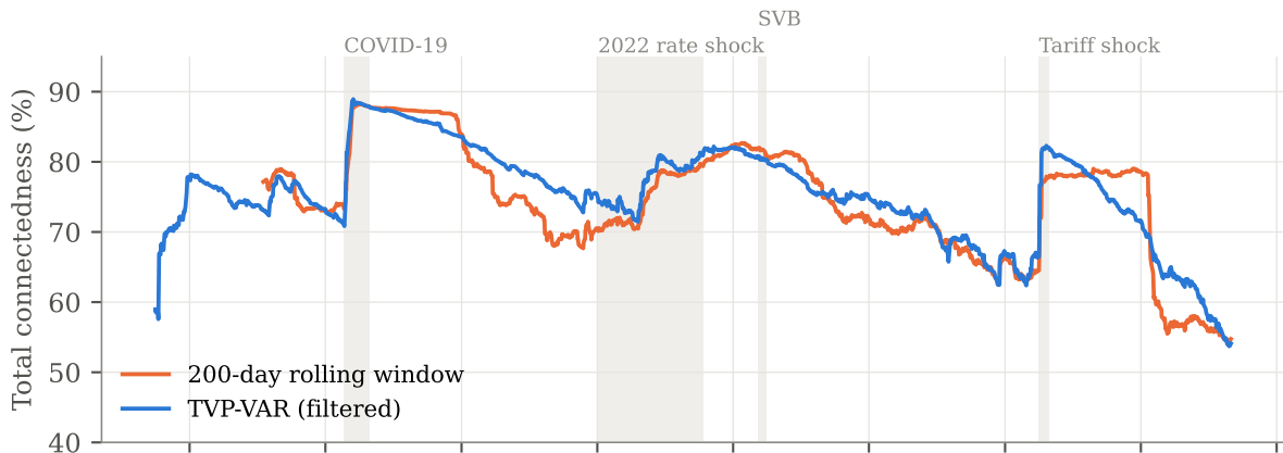
(b) Volatility connectedness, TVP-VAR (filtered)
