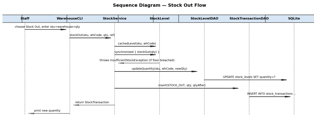
Figure 5 — Sequence diagram: Stock Out
