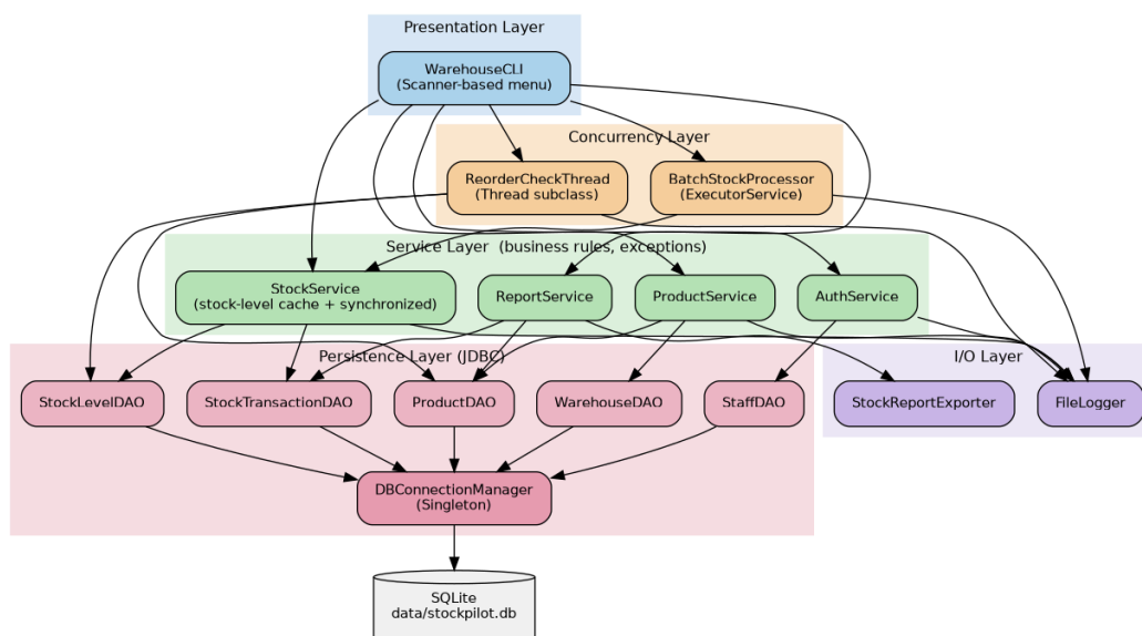
Figure 2 — Layered system architecture
