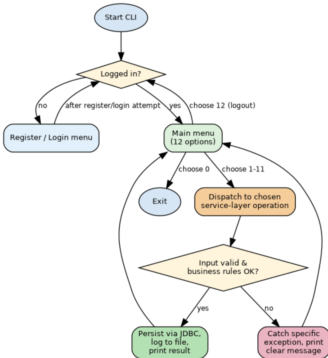
Figure 1 — CLI menu / process-flow diagram
