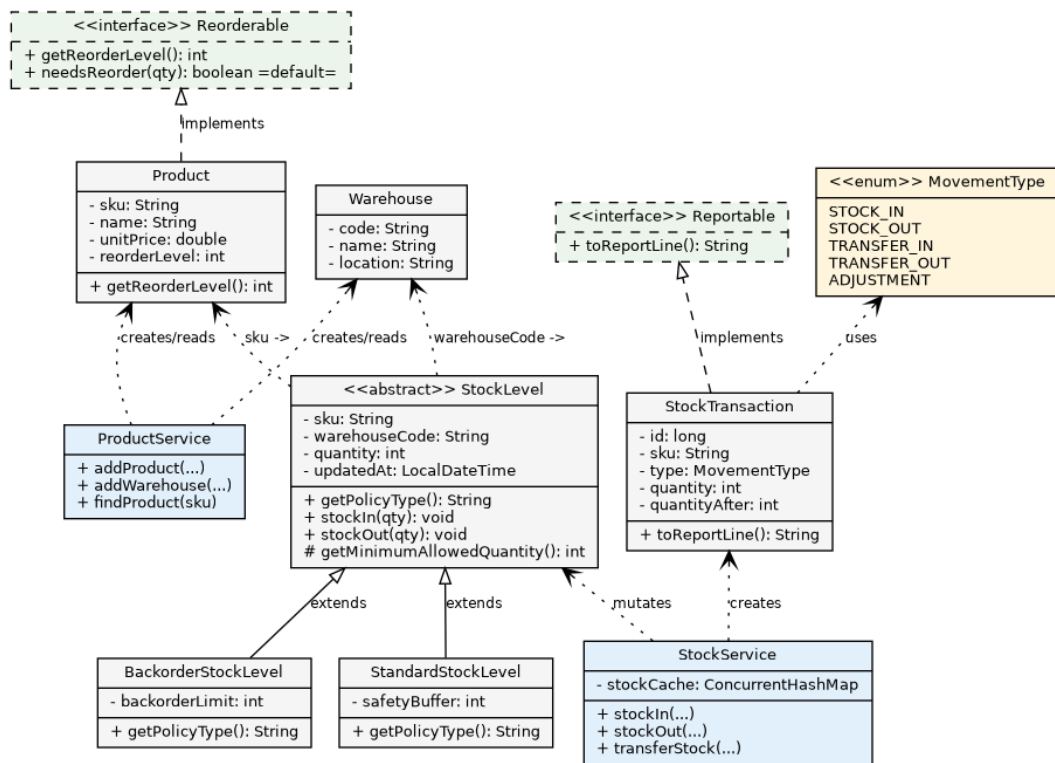
Figure 4 — Class diagram (core model + representative services)
