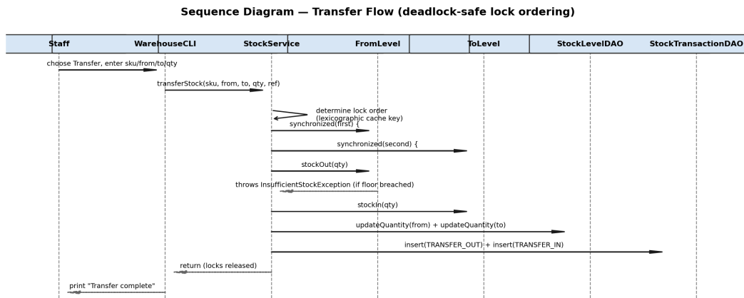
Figure 6 — Sequence diagram: Transfer
