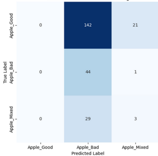
Confusion Matrix Before Training
