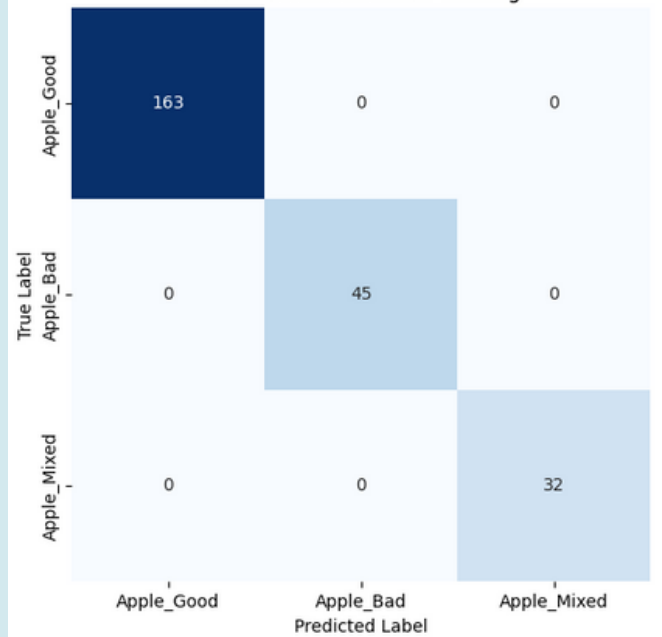
Confusion Matrix After Training
