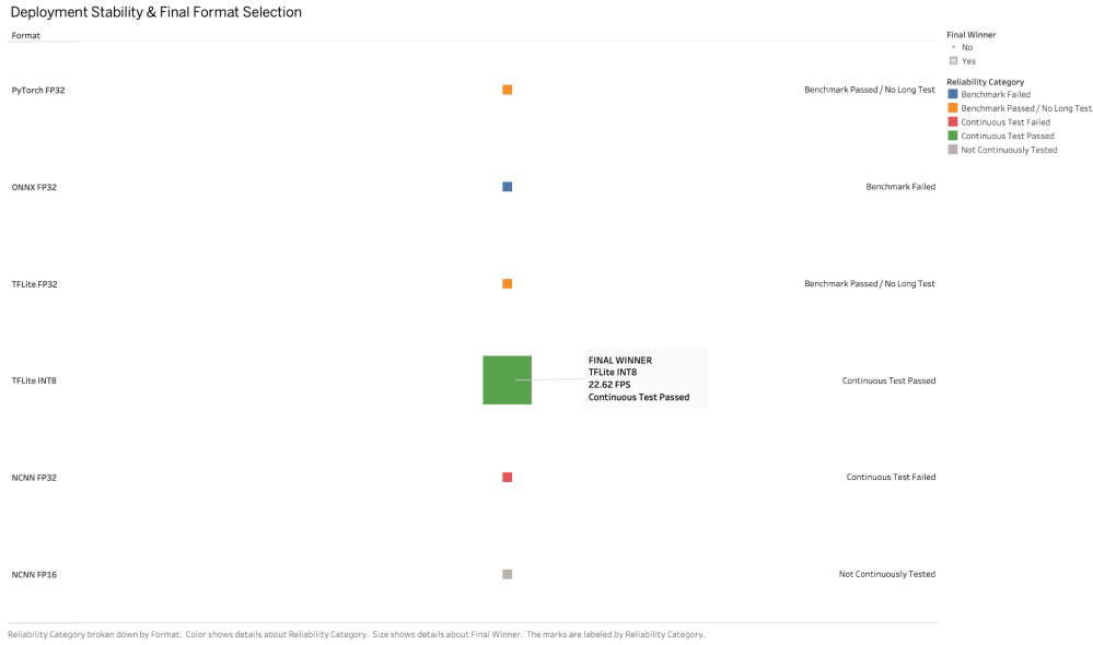
Figure 4.6: Operational-status comparison across exported formats, distinguishing fixed-benchmark completion from continuous-test outcomes. TFLite INT8 is the only format with both a completed benchmark and a valid continuous run, supporting its final selection.
