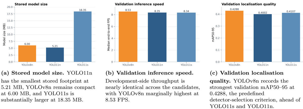
Figure 3.7: YOLO candidate efficiency and validation quality.
