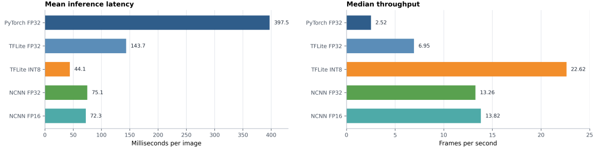
(a) Runtime performance: mean inference latency and median throughput for the five completed representations.
