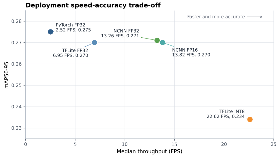
Figure 4.2: Median throughput plotted against mAP50–95 for each deployment format that completed the Raspberry Pi benchmark. Points farther right are faster and points higher on the chart retain stronger localisation quality; ONNX FP32 is omitted because no valid aggregate benchmark was completed.
