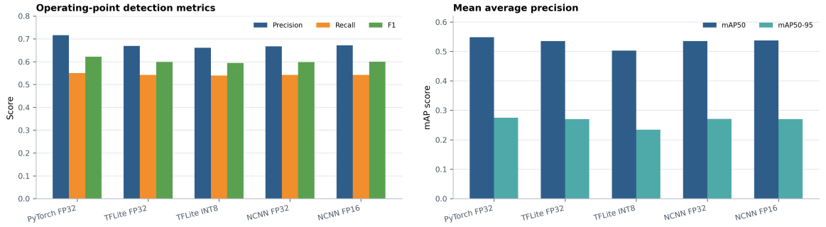
(c) Detection quality: precision, recall, F1, mAP50 and mAP50-95 retained after deployment conversion.
