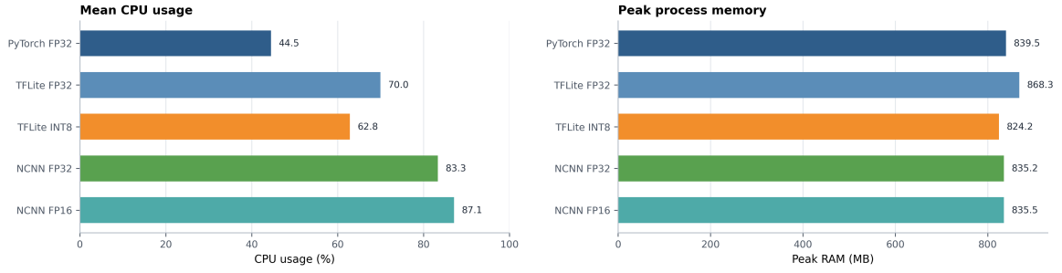
(b) Resource demand: mean CPU usage and peak process memory measured during the same 90-image benchmark.
