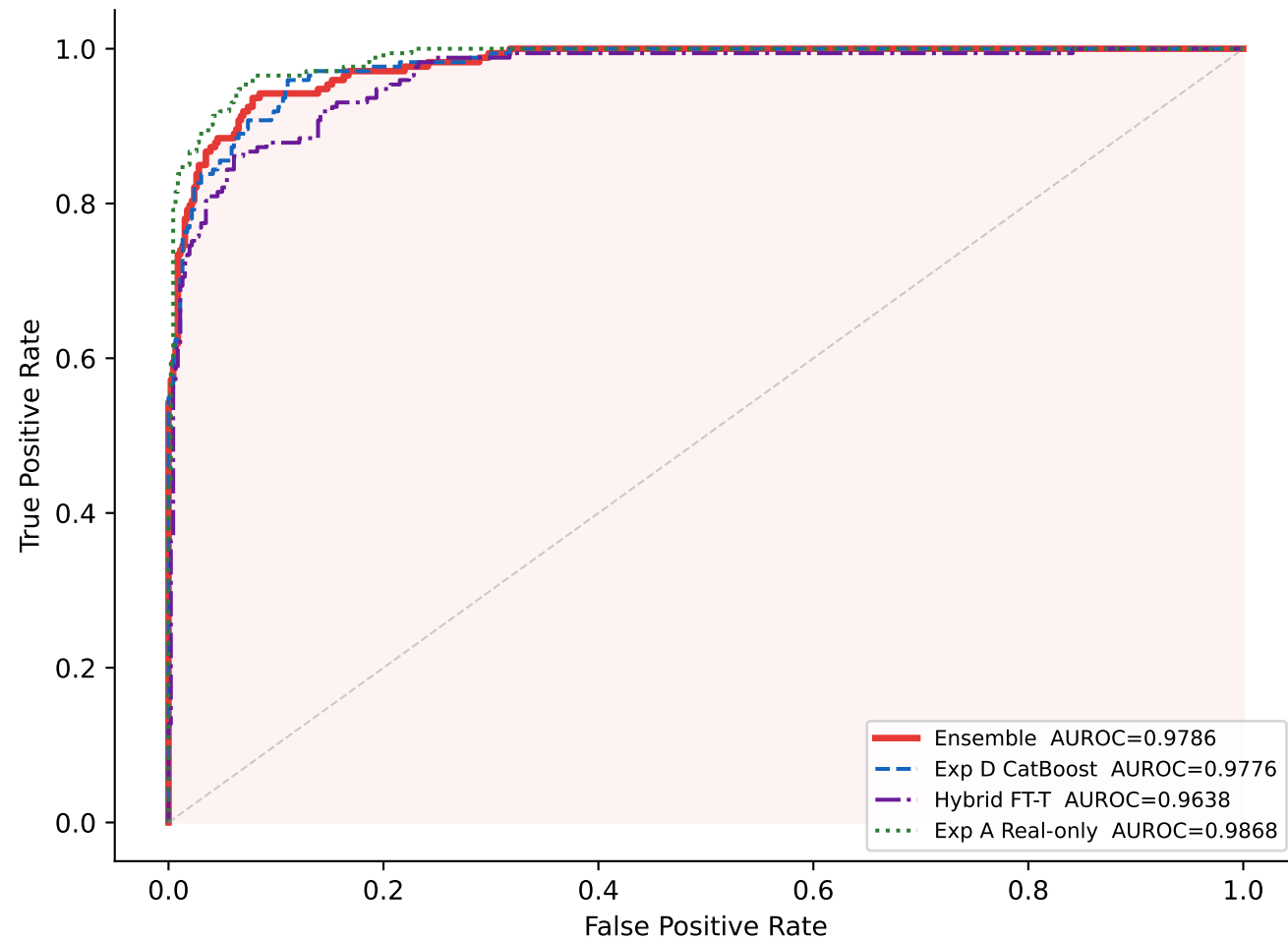
ROC Curve
