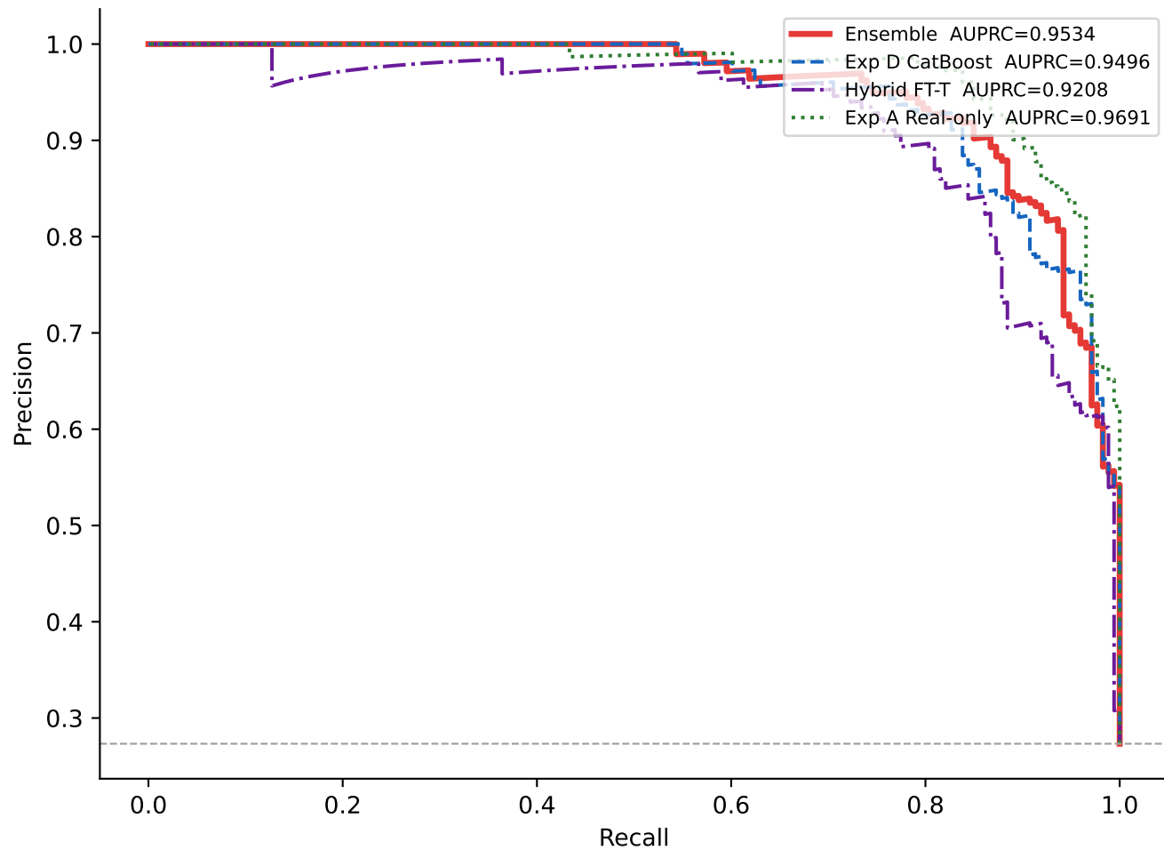
Precision-Recall Curve
