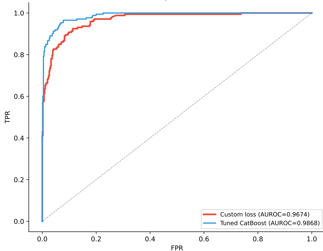
ROC — Custom Loss vs Tuned CatBoost Option B
