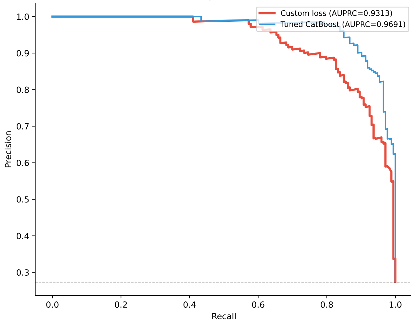
PR — Custom Loss vs Tuned CatBoost Option B
