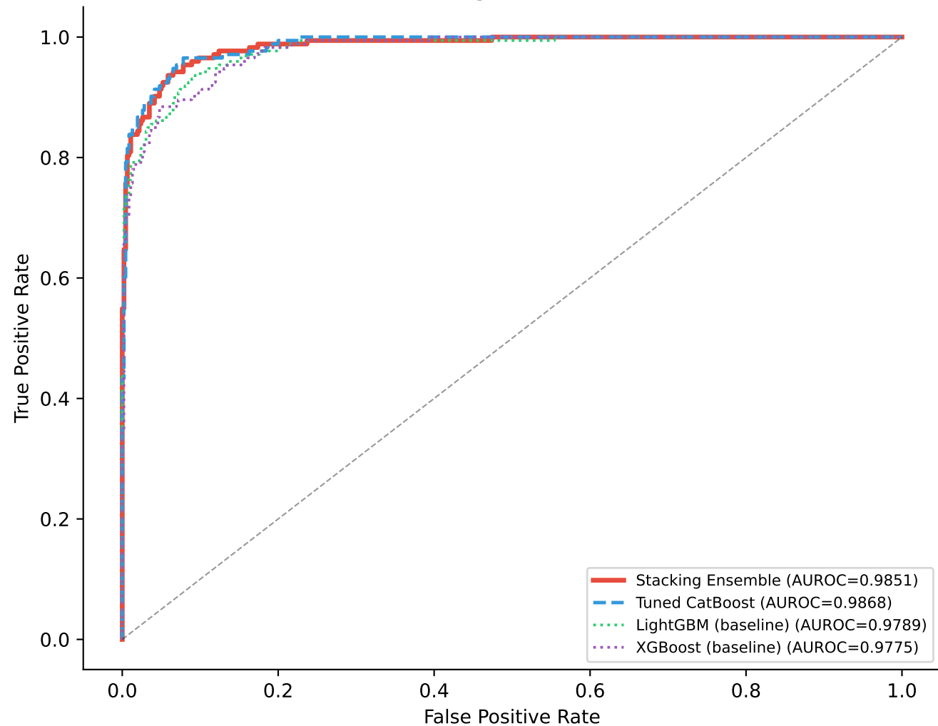
ROC — Stacking Ensemble vs All Option B
