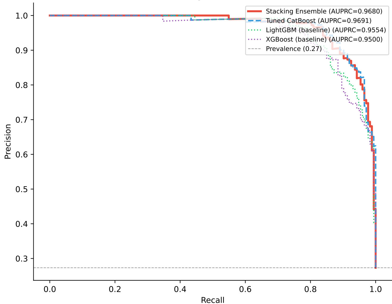
Precision-Recall — Stacking Ensemble vs All Option B
