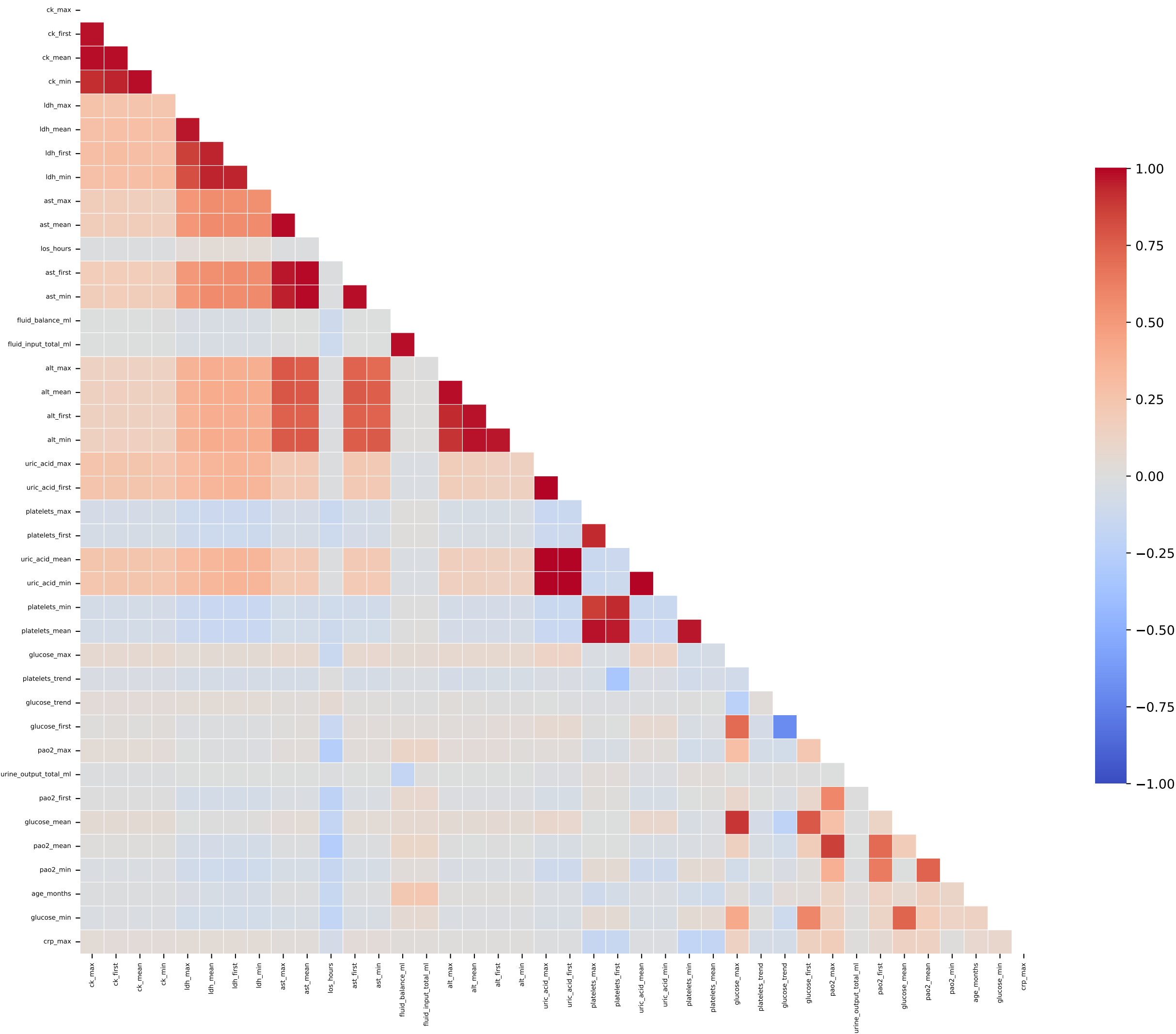
Feature correlation heatmap — top 40 variables by variance
