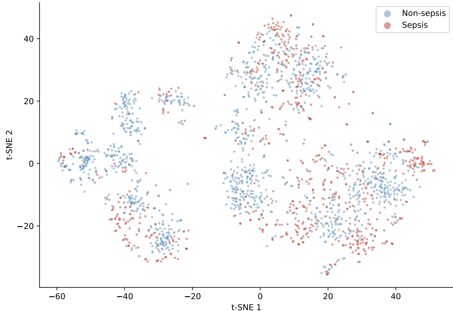
t-SNE feature-space visualisation — Option A — Full cohort (sample n=2000; interpret overlap to decide on SMOTE)
