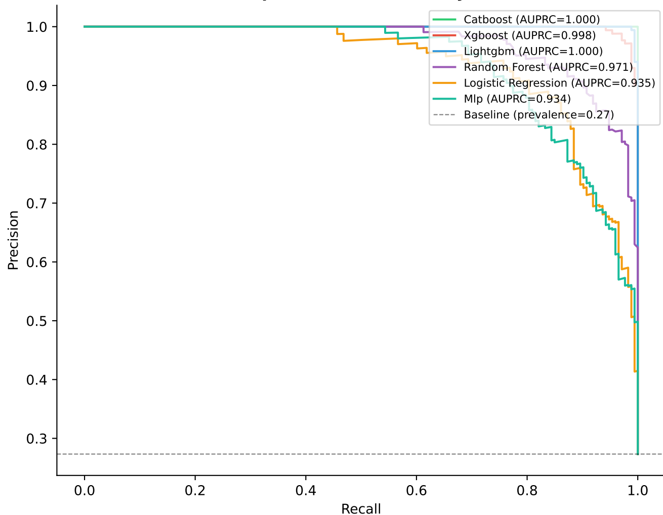
Precision-Recall Curves — All Models Option B (Infection-only)
