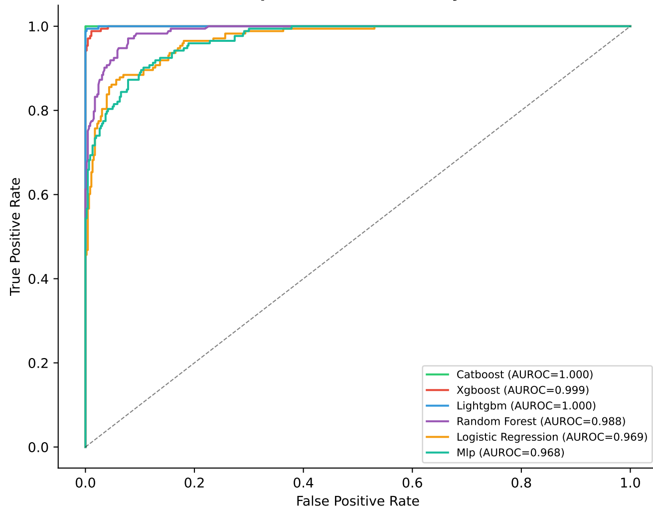
ROC Curves — All Models Option B (Infection-only)
