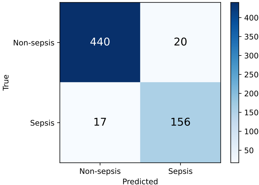
Stacking Ensemble — Confusion Matrix Sens=0.9017 Spec=0.9565 Thresh=0.1882
