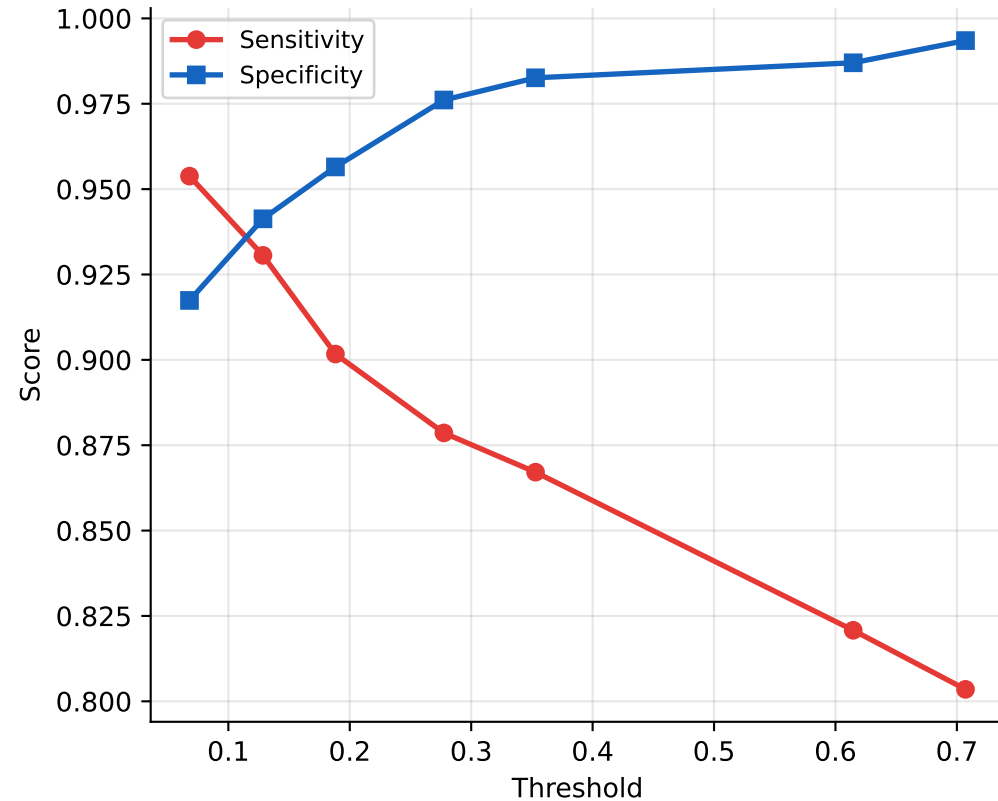
Sensitivity vs Specificity
