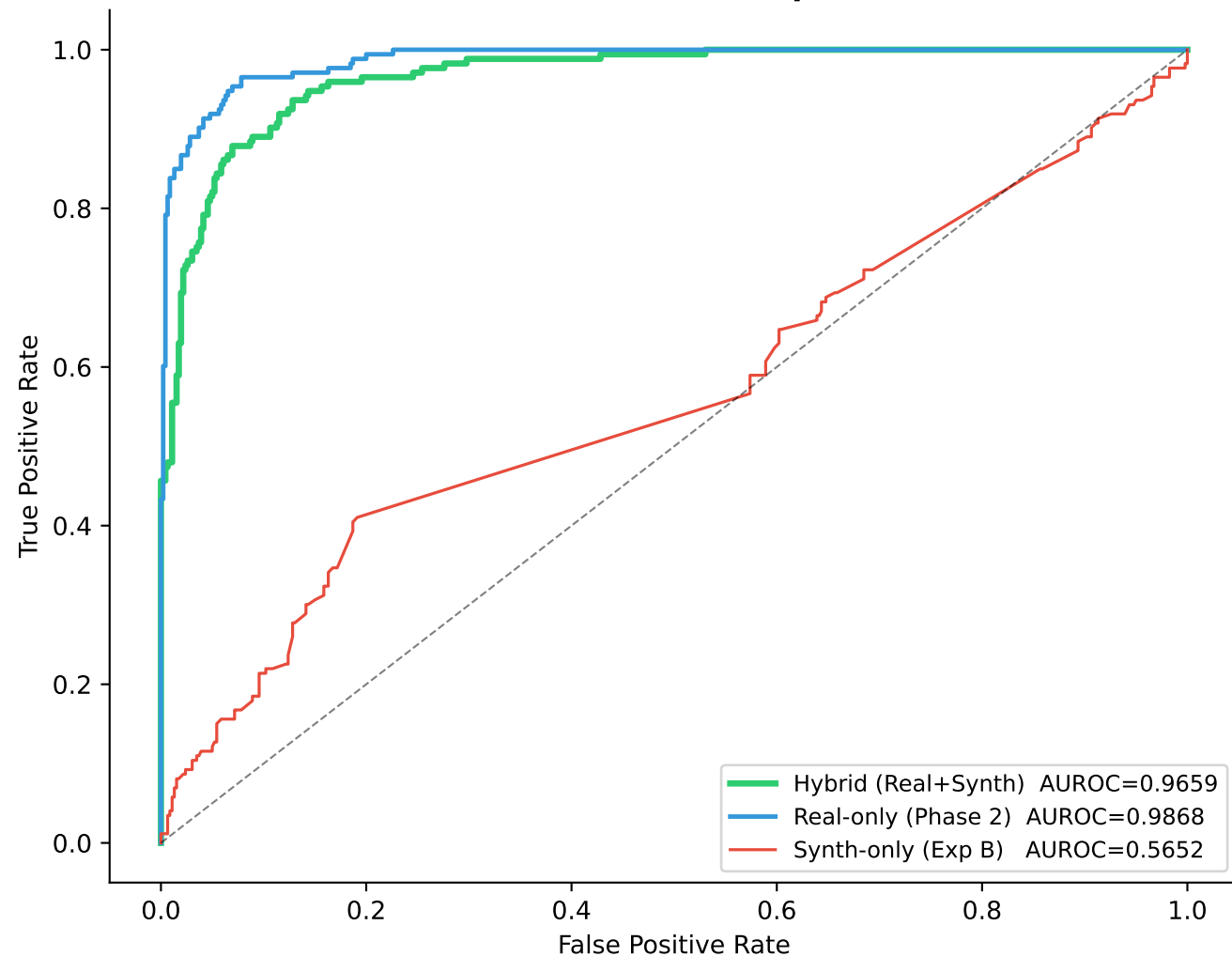
ROC — Hybrid vs Synthetic-only vs Real-only Evaluated on Real Test Set (Option B, n=633)
