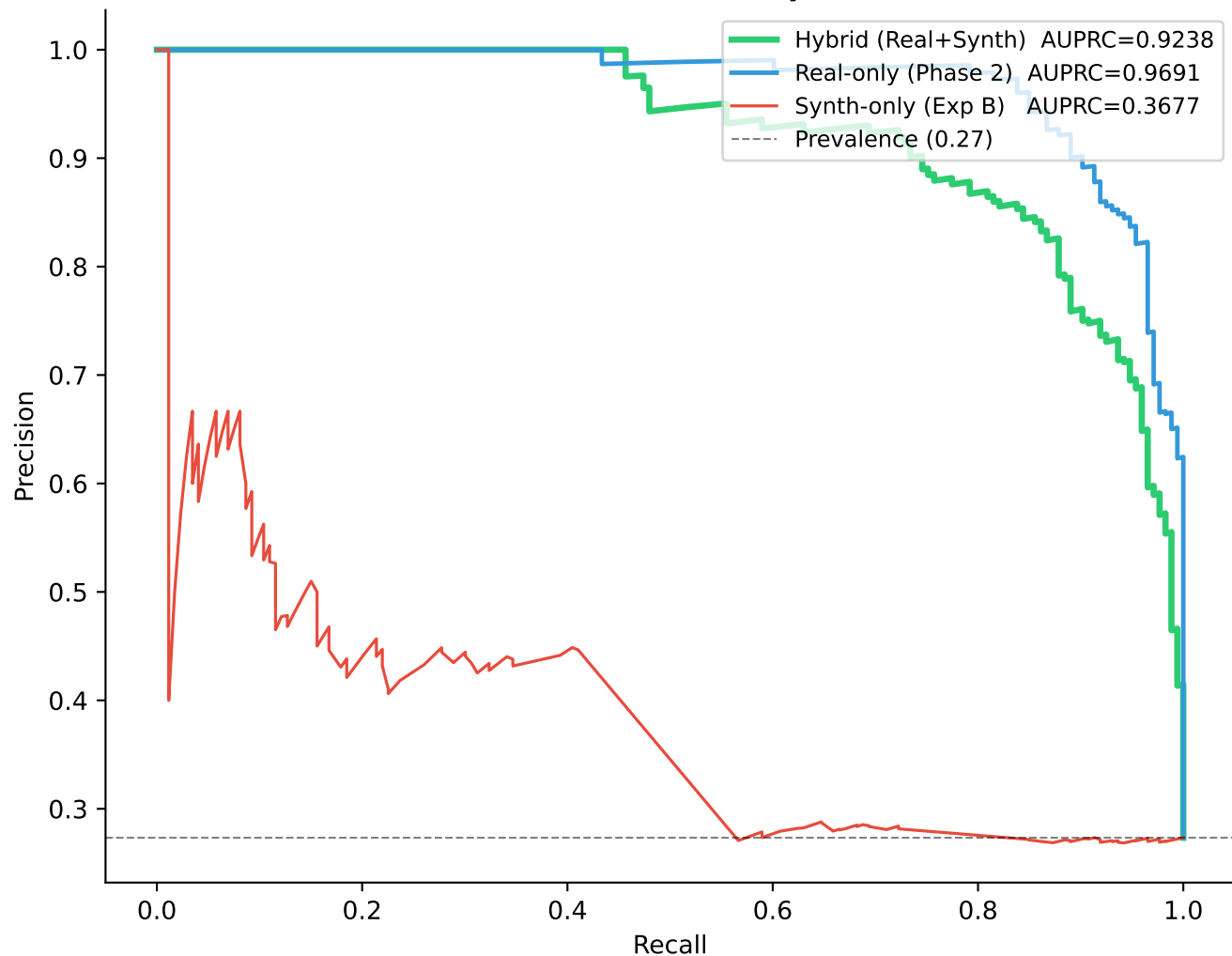
Precision-Recall — Hybrid vs Synthetic-only vs Real-only Evaluated on Real Test Set (Option B, n=633)
