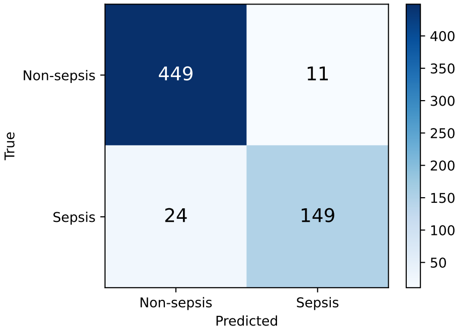
Confusion Matrix — Random Forest Sens=0.861 Spec=0.976 Threshold=0.472
