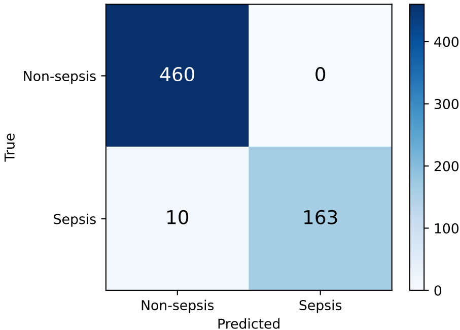
Confusion Matrix — Xgboost Sens=0.942 Spec=1.000 Threshold=0.866
