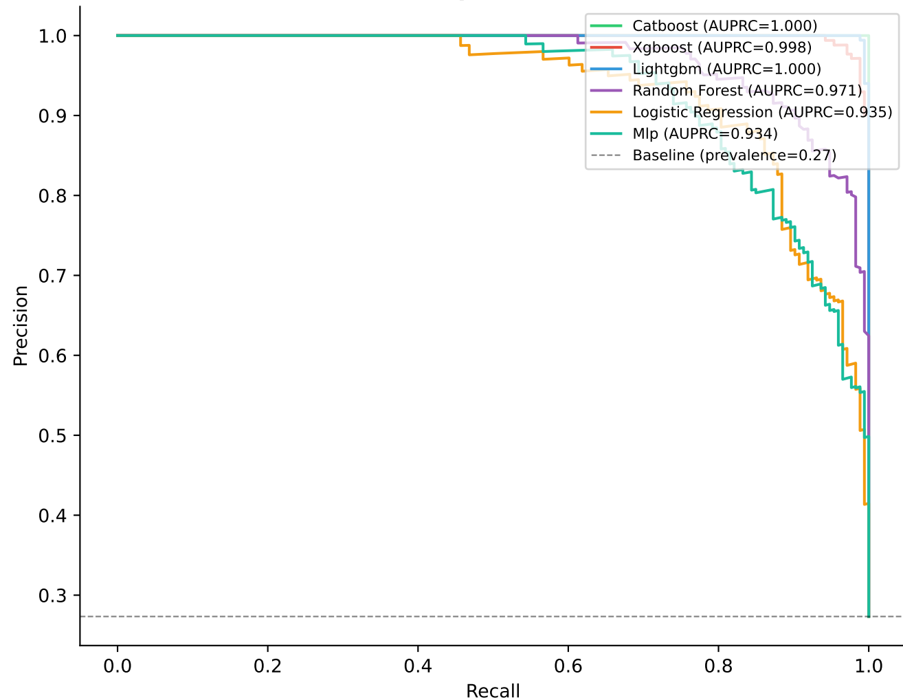
Precision-Recall Curves — All Models Option B
