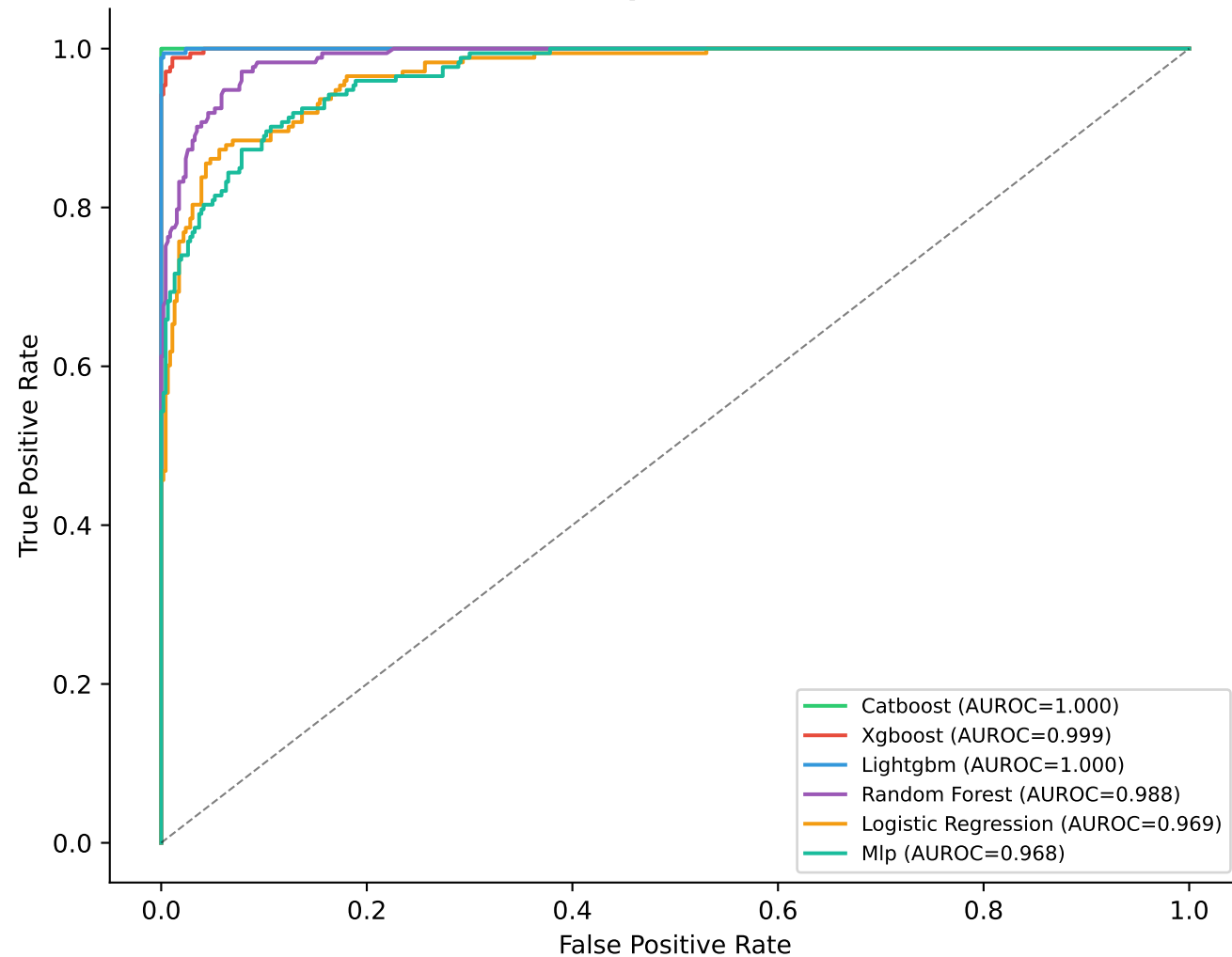
ROC Curves — All Models Option B
