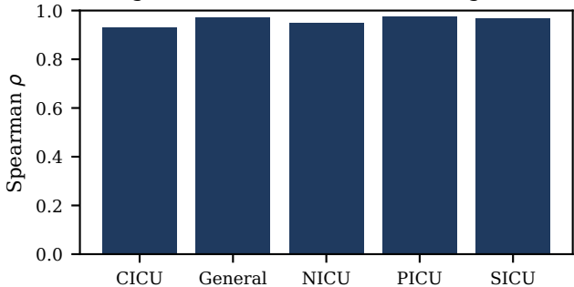
Node agreement with federated ranking (FEDAVG)
