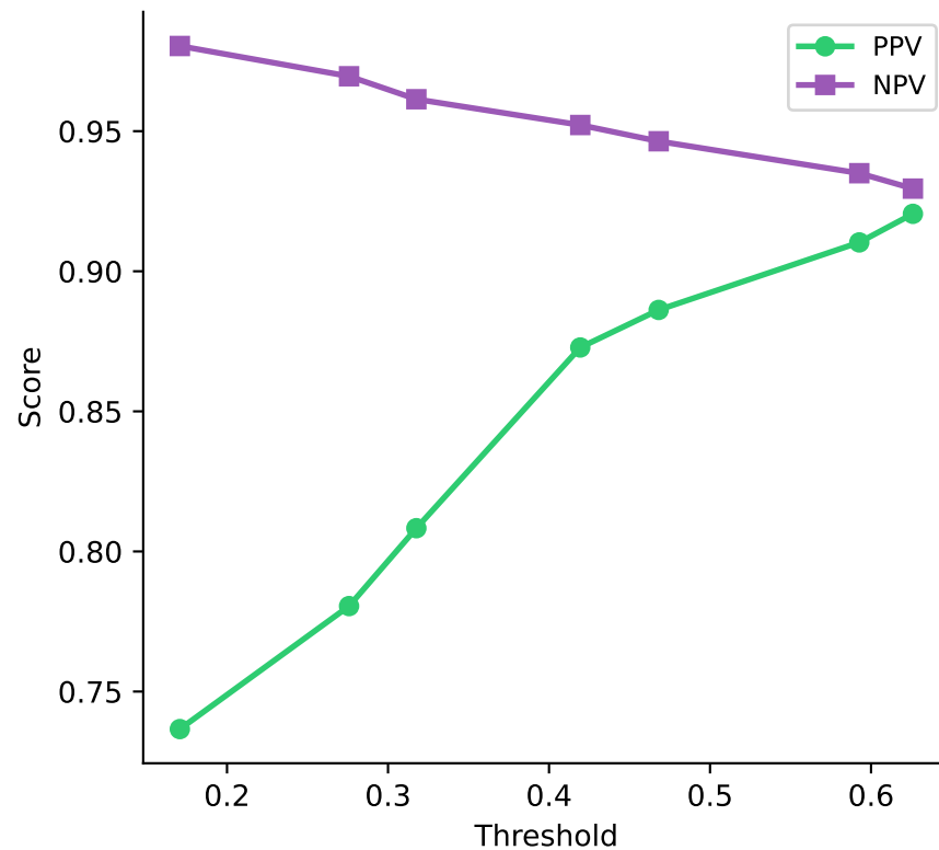
PPV vs NPV
