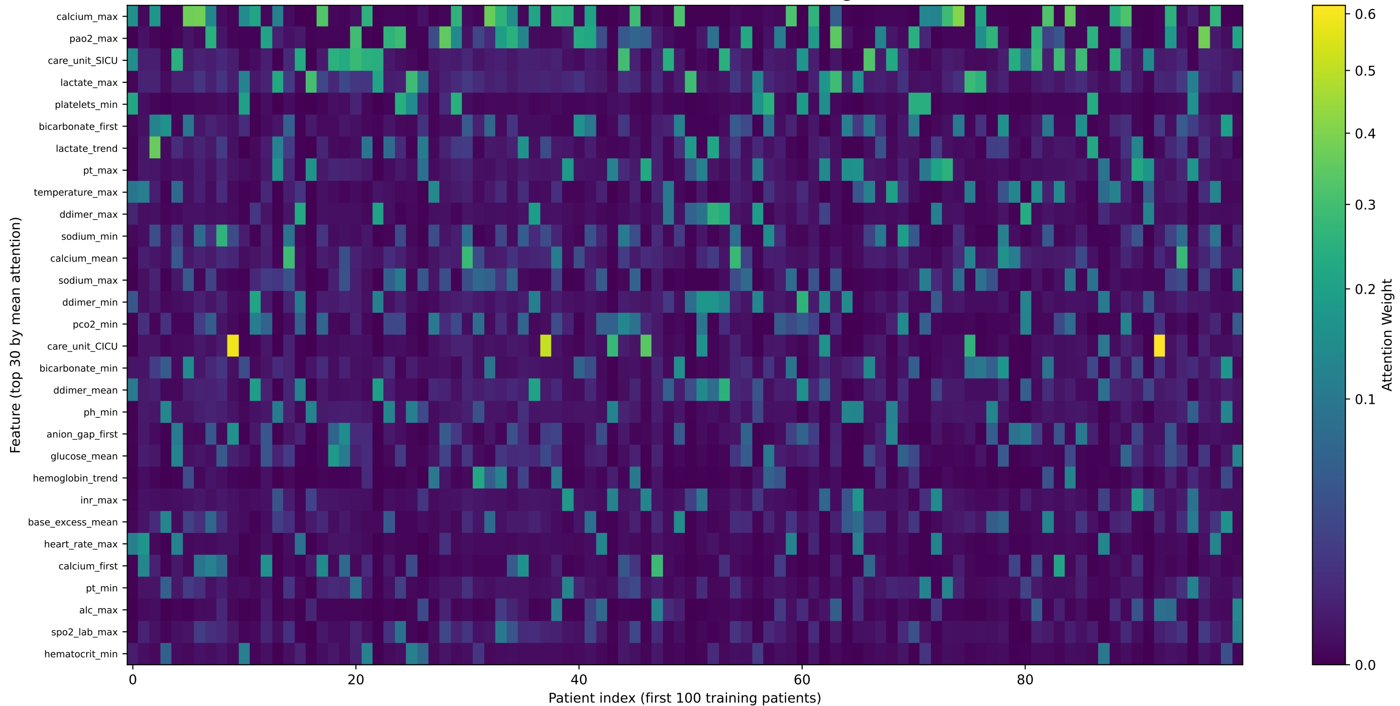
FT-Transformer Attention Weights — Top 30 Features x First 100 Patients Last block, CLS-token row, head-averaged
