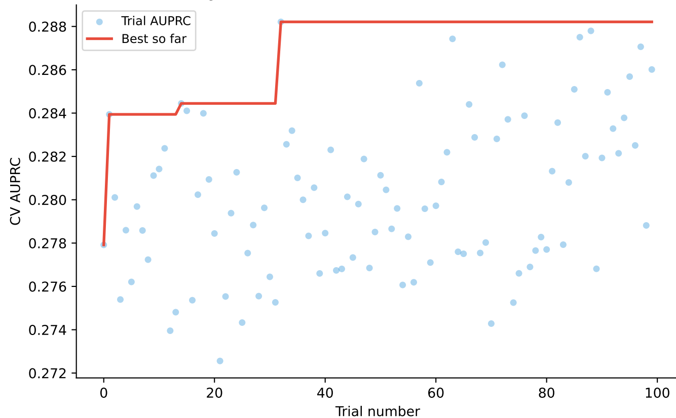
Optuna optimization history Synthetic-trained CatBoost — 100 trials
