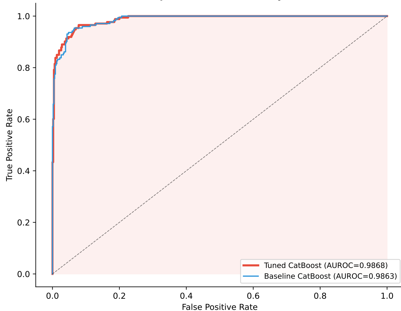
ROC — Tuned vs Baseline CatBoost Option B (Infection-only)
