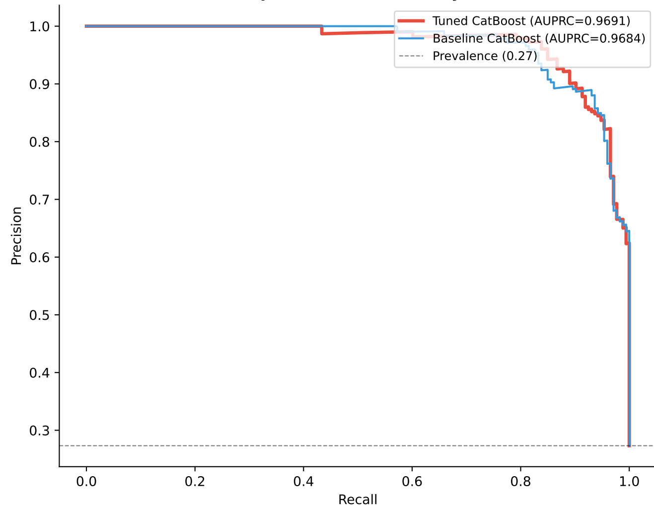
Precision-Recall — Tuned vs Baseline CatBoost Option B (Infection-only)
