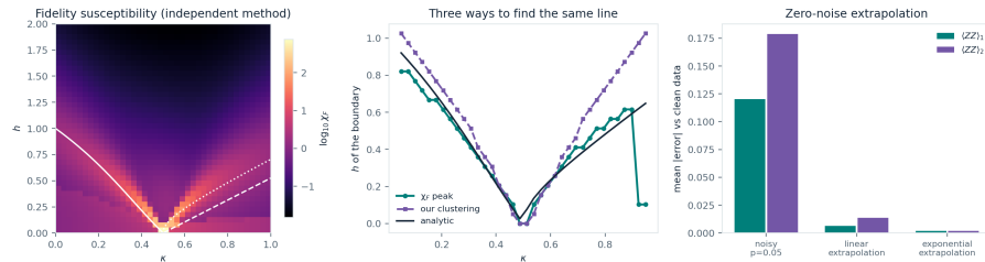
Fidelity susceptibility, computed without any classifier; the boundary located three independent ways; extrapolation error against clean data.
